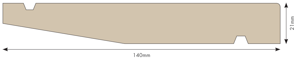
Bevel Back – Imperial Profile 140mm x 21mm (Cover 108mm)
