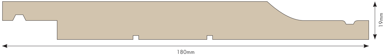
Scallop Rusticated – 180mm x 19mm (Cover 155mm)
