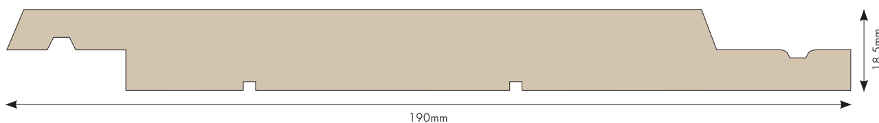
Vertical Shiplap – 190mm x 18.5mm (Cover 165mm)
