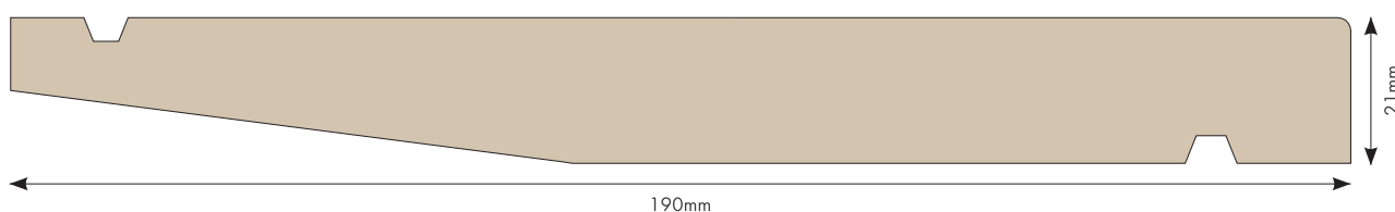
Bevel Back – 190mm x 21mm (Cover 148mm)
