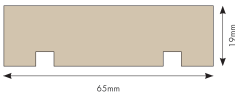
Batten – 65mm x 19mm (Also available in 40mm x 19mm & 90mm x 19mm)
