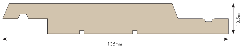
Vertical Shiplap – 135mm x 18.5mm (Cover 110mm)
