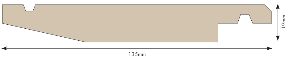
Rebated – 135 x 19mm (Cover 110mm)
